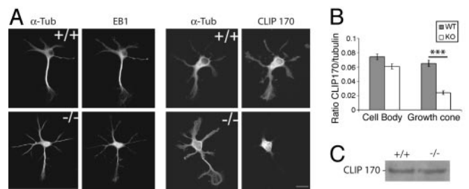
Fig. 6. Distribution of EB1 and CLIP170 in hippocampal neurons. (A) Double-immunofluorescence of EB1/ \alpha -tubulin and CLIP170/ \alpha -tubulin in WT and TTL null neurons. In both, EB1 is distributed throughout the cell body, neurites, and growth cones with a characteristic "comet" pattern. In WT neurons, CLIP170 is also distributed throughout the cell body, neurites, and growth cones, whereas in TTL null neurons, the CLIP170 signal is restricted to the cell body and initial parts of neurites, being undetectable in growth cones (see Fig. 10 for higher magnification). (Scale bar: 10 \mu m.) (B) Quantitative analysis of CLIP170 staining, showing CLIP170/ \alpha -tubulin fluorescence intensity ratios in cell bodies (WT, n = 32 ; TTL null, n = 41 ) or growth cones from WT or TTL null neurons (WT, n = 30 ; TTL null, n = 27 ). Growth cones of TTL null neurons showed a significant reduction in CLIP170 levels compared with WT cells. ***, P < 0.001 (t test). (C) Immunoblot analysis of CLIP170 content in WT or TTL null neurons. Equal amounts of total protein were loaded.
