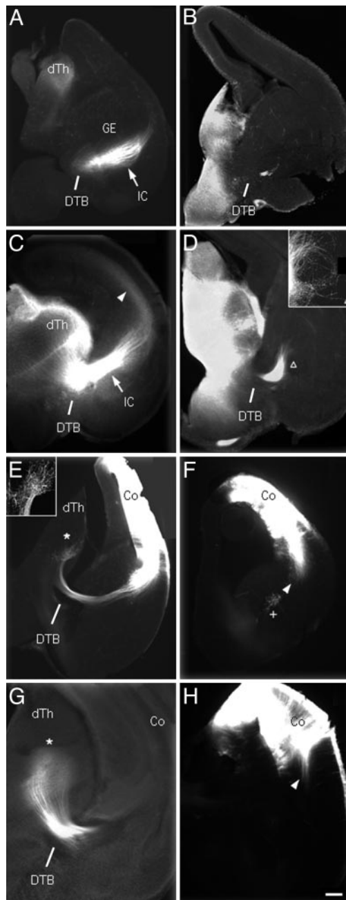
Fig. 4. Defective cortico-thalamic loop in embryonic TTL null mice. Dil labeling of the cortico-thalamic loop at E15 (A, B, E, and F) and E17 (C, D, G, and H) in WT (Left) or TTL null (Right) embryos, axon labeling after dil implants in the thalamus (A–D) or the cortex (E–H). (A) In E15 WT embryos, labeled thalamo-cortical axons grew through the IC (white arrow) up to the intermediate zone of the ventral cortex. (B) In contrast, in E15 TTL null embryos, a small bundle of labeled fibers just crossed the DTB, but did not form an IC. (C) In E17 WT embryos thalamo-cortical axons formed a thick bundle in IC (white arrow), and leading fibers reached their maximum extent in the intermediate zone of the dorsal cortex (white arrowhead). (D) In E17 TTL null embryos diI-labeled axons failed to form an IC, but wandered about in a looping trajectory (triangle and Inset ). (E) Cortico-thalamic axons in E15 WT embryos formed a dense terminal projection zone in the thalamus (white star and Inset ). (F) In E15 TTL null embryos, the maximum extent of labeled axons was restricted to the neocortex (white arrowhead). (G) In E17 WT embryos, labeled cortico-thalamic axons elaborate a dense terminal field (white star) whereas (H) in TTL null embryos the maximum extent reached by labeled axons is still confined to the neocortex as shown at E15 (compare white arrowheads in F and H). Co, cortex; dTh, dorsal thalamus. (Scale bar: 150 \mu m, A–F; 60 \mu m, Insets in D and E; and 75 \mu m, G and H.)
