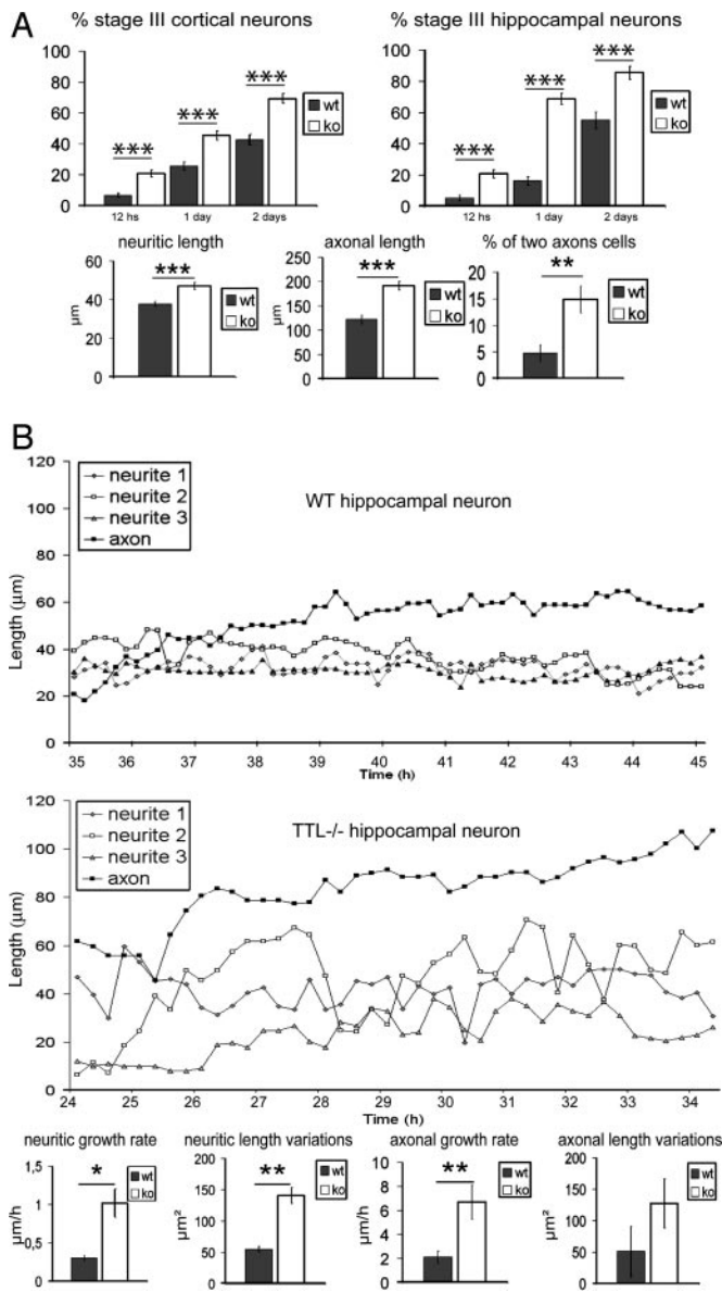
Fig. 5. Neurite outgrowth and axonal differentiation in cultured neurons. (A) Cell differentiation of cortical and hippocampal neurons in WT or TTL null primary culture after 0.5, 1, and 2 days in vitro . The percentage of cells reaching stage III (presence of an axon) was always increased in TTL null cells compared with WT cells, indicating a premature differentiation of TTL null neurons. Compared with WT cells in 2-day in vitro hippocampal cells, both neurite (WT, n = 150 ; TTL null, n = 110 ) and axonal (WT, n = 50 ; TTL null, n = 75 ) mean length were longer in TTL null cells. TTL null cultures also revealed a higher percentage of cells with two axon-like processes ( n = 190 for both WT and TTL null). (B) Morphological changes during establishment of polarity in cultured hippocampal neurons examined by time-lapse, phase-contrast video microscopy. Neurite and axon growth was examined from 1 day after plating until 3 days, showing a 10-h sequence window including the phase of axon formation. Because axon differentiation is premature in TTL null cells, this window corresponds to different time points in WT and TTL null cultures. Quantification was performed by using the complete data. In WT hippocampal neurons, neurites extended and retracted over short distances over time. In TTL null neurons, neurites extended or retracted over markedly longer distances. The net rate of neurite (WT, n = 16 ; TTL null, n = 18 ) and axonal (WT, n = 9 ; TTL null, n = 10 ) elongation was increased in TTL null cells compared with WT cells. Neuritic length variations (measured as the linked variance of neuritic length around the linear regression of length vs. time) were significantly higher in TTL null neurons compared with WT neurons.
